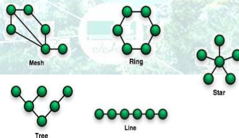
Network Topology
